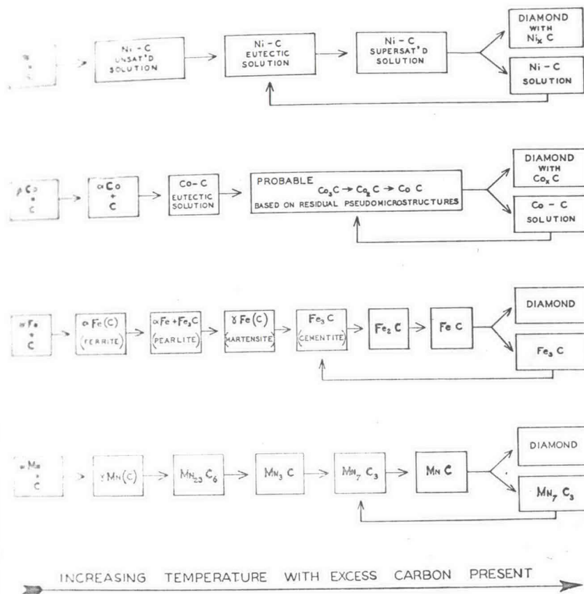
FIG. 8. A flow diagram illustrating the sequential nature of metal-carbon interaction (in an excess of carbon) under high pressure as a function of temperature. The designated presence of Fe 2 C is tentative.
